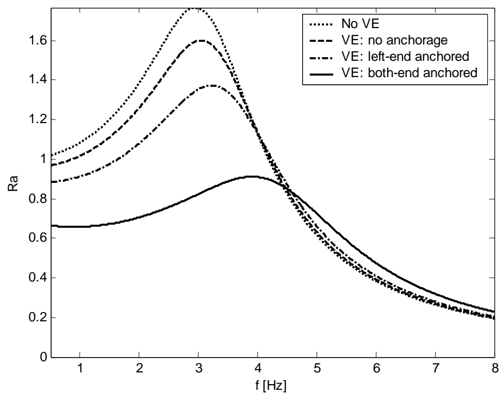
Fig. 9. Acceleration ratio for a simply supported beam for different configurations of VE layers with t_v equal to 0.32 cm including no VE layer case. The results are shown for a beam with 51 cm thickness.
