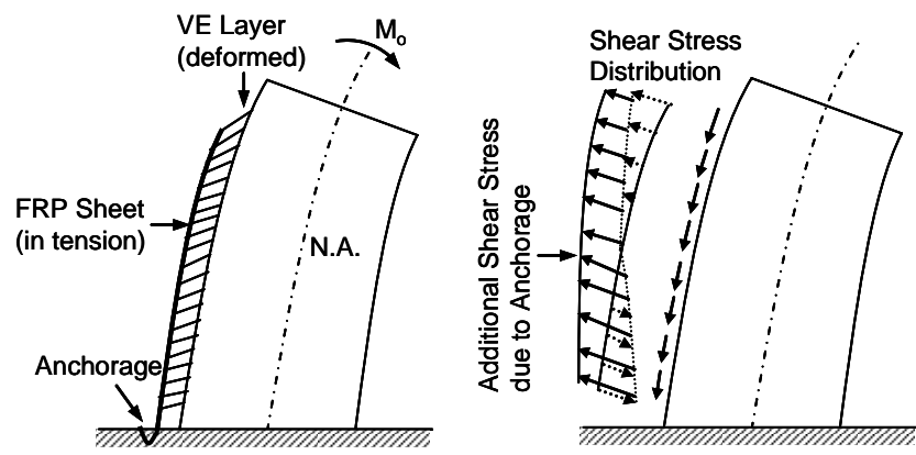
(b) Anchored constrained layer.
