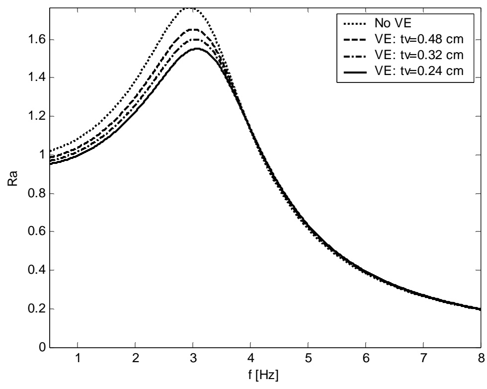
Fig. 11. Acceleration ratio for a simply supported beam with no anchorage case for different thickness of VE layers including no VE layer case. The results are shown for a beam with 51 cm thickness.
