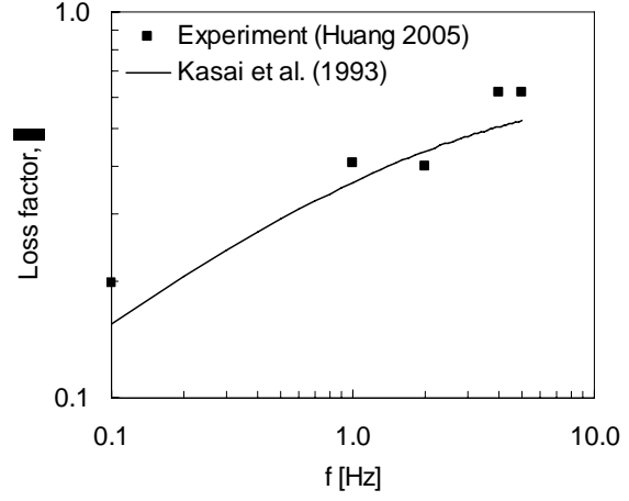
(b) Loss factor.
